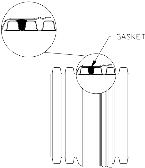
BELL & SPIGOT JOINT 4" - 8" (100-200 MM)
