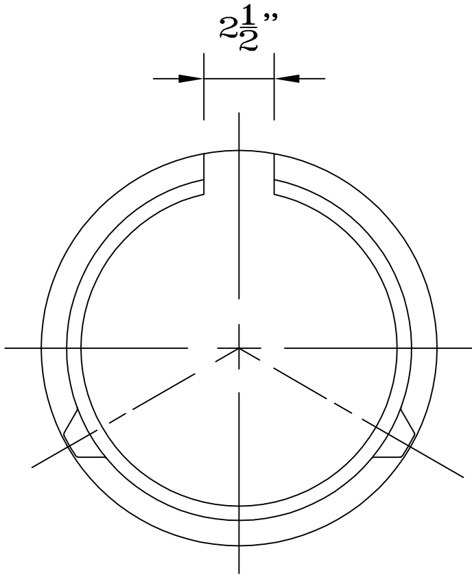
END VIEW
