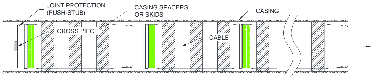
Figure 3 Alternative Installation Method (Used when maximum insertion forces are likely to be exceeded)
