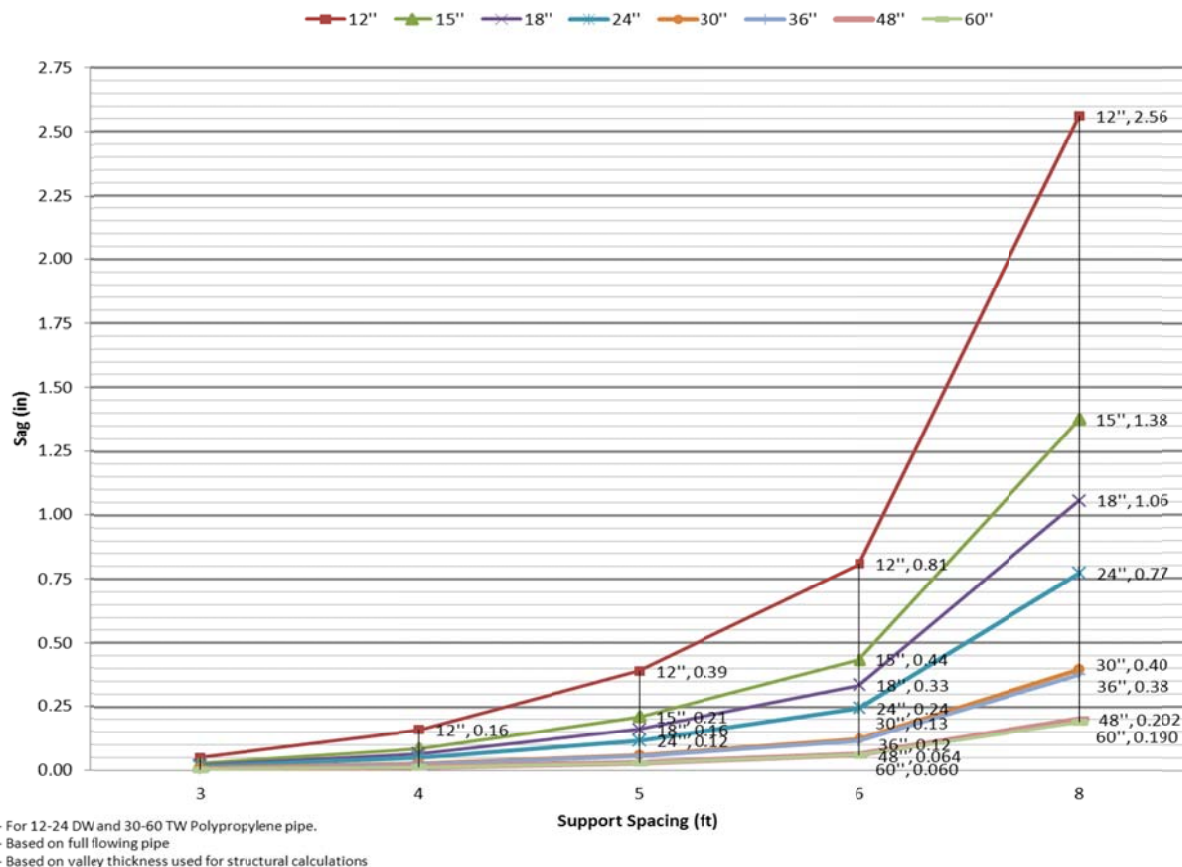
Chart 1 Unsupported Deflection of SaniTite HP
